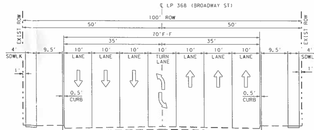
EXISTING LP 368 (100' ROW)
