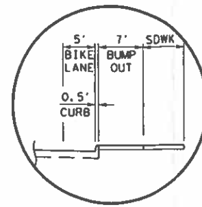
DETAIL "A" - BUMPOUT DETAIL
