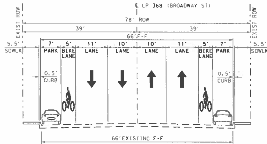
PROPOSED LP 368 (78' ROW)
