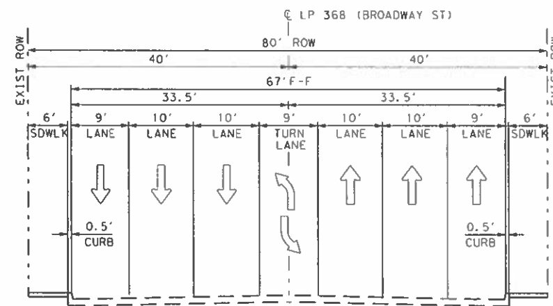
EXISTING LP 368 (80' ROW)
