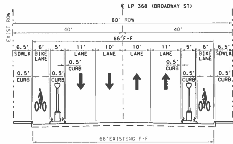
PROPOSED LP 368 (80' ROW)
