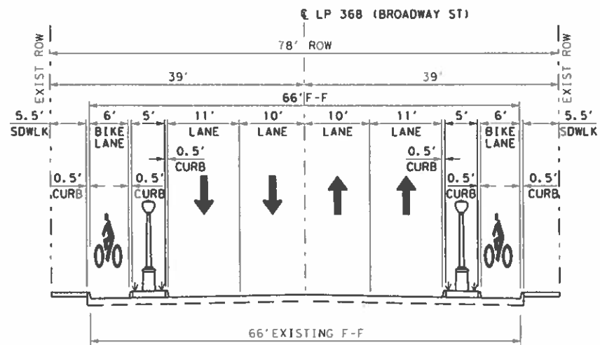
PROPOSED LP 368 (78' ROW)
