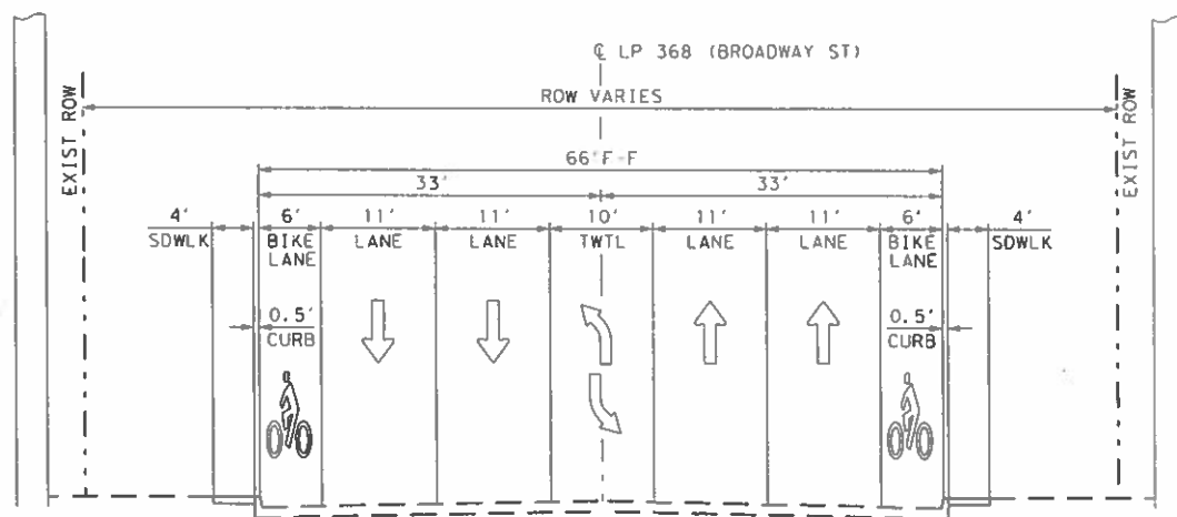
EXISTING LP 368 (ROW VARIES)
