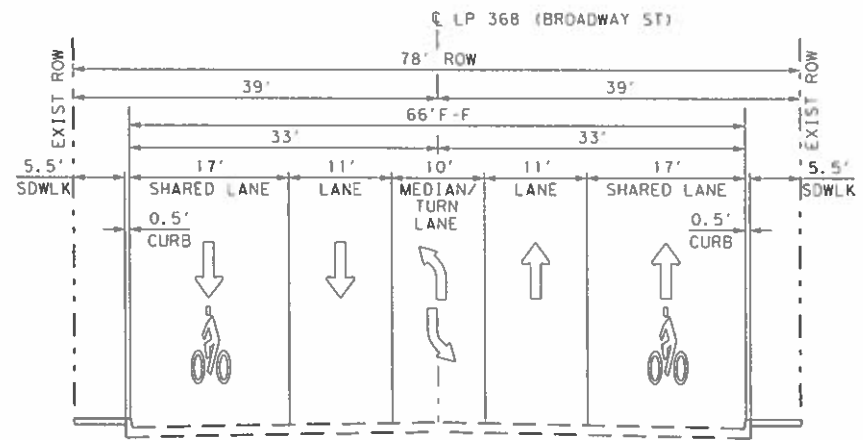
EXISTING LP 368 (78' ROW)
