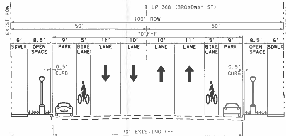
PROPOSED LP 368 (100' ROW)
