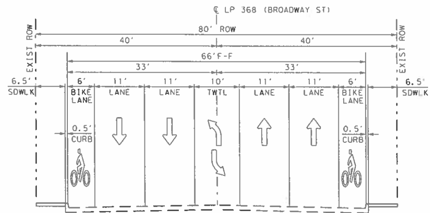
EXISTING LP 368 (80' ROW)
