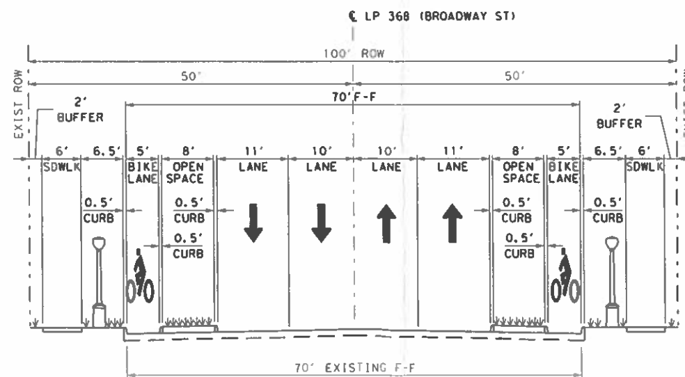
PROPOSED LP 368 (100' ROW)
