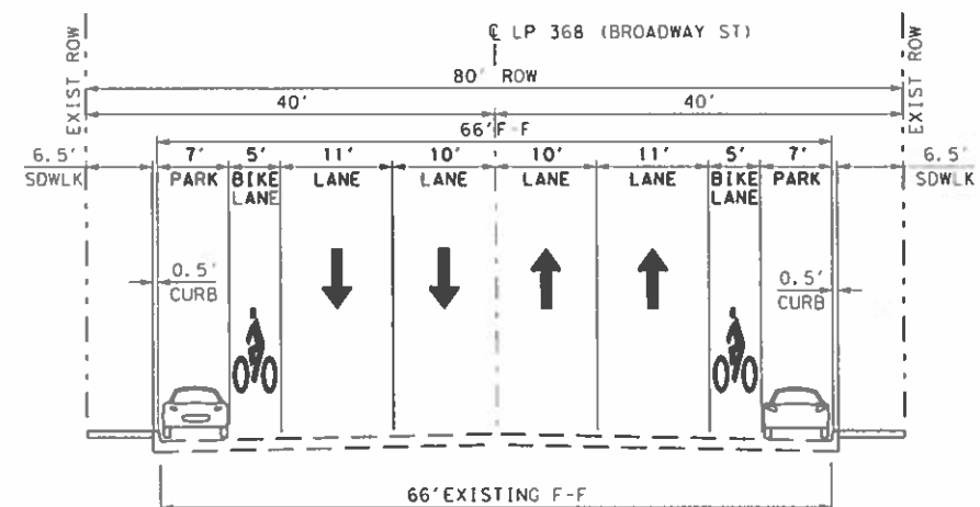
PROPOSED LP 368 (80' ROW)
