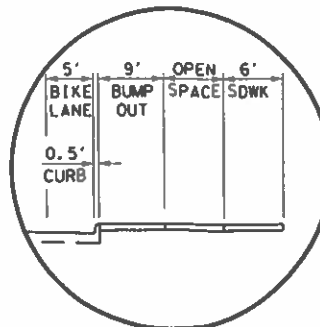
DETAIL "B" - BUMPOUT DETAIL
